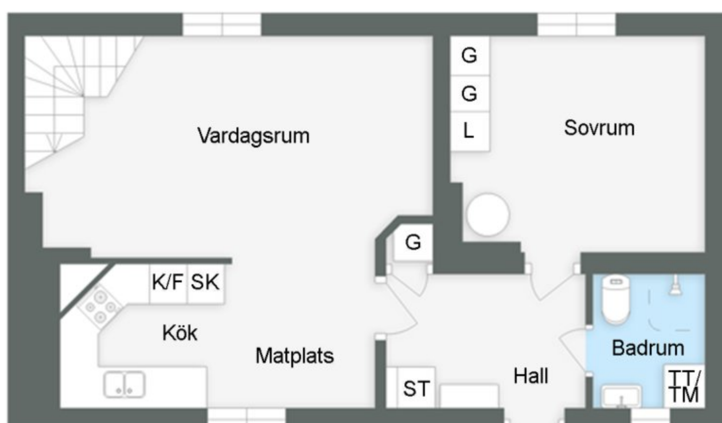
Plan 1
